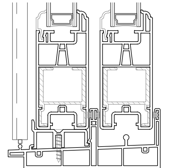
5 Sill Detail
