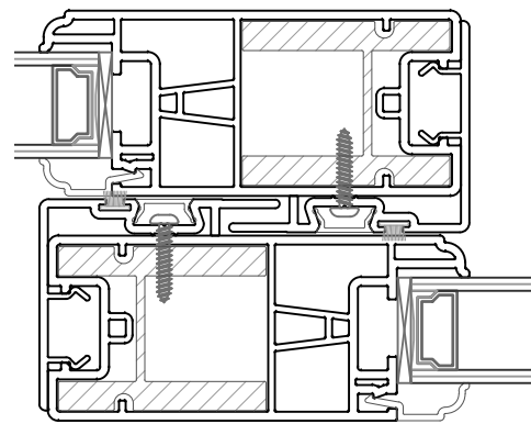
7 Meeting Rail Detail
