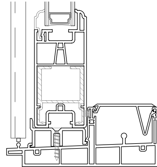
2 Sill Detail
